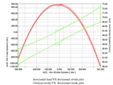
Dynamic tests for the Sliding Pendulum Isolators for the Bursa Hospital, Turkey, executed in our laboratory
