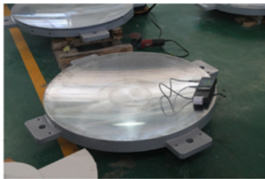
SUPPLY AND INSTALLATION OF 600 HISLIDE PENDULUM DEVICES (VERTICAL LOAD 1000KN ) FOR SEBES – TURDA MOTORWAY, ROMANIA
